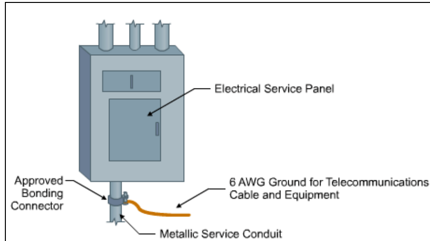
Figure 1 Bonding
