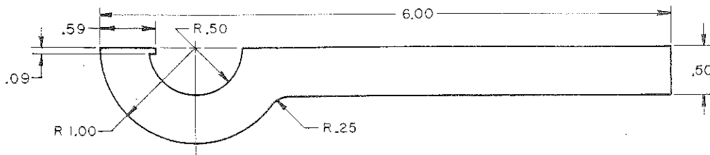
SPANNER WRENCH
