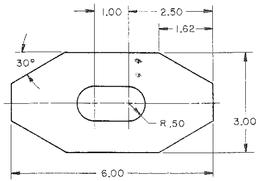
STRAP CLAMP
